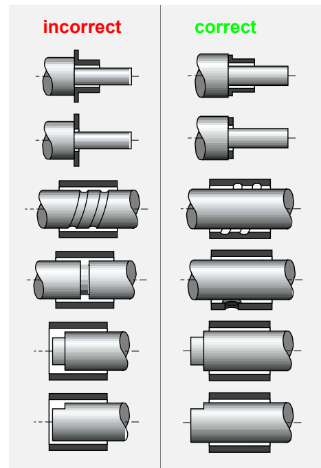
Fig. 25: Counterface Design
