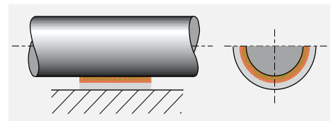
Fig. 20: Boundary lubrication
