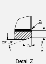
Dimensions and Tolerances according to ISO 3547 and GSP-Specifications
